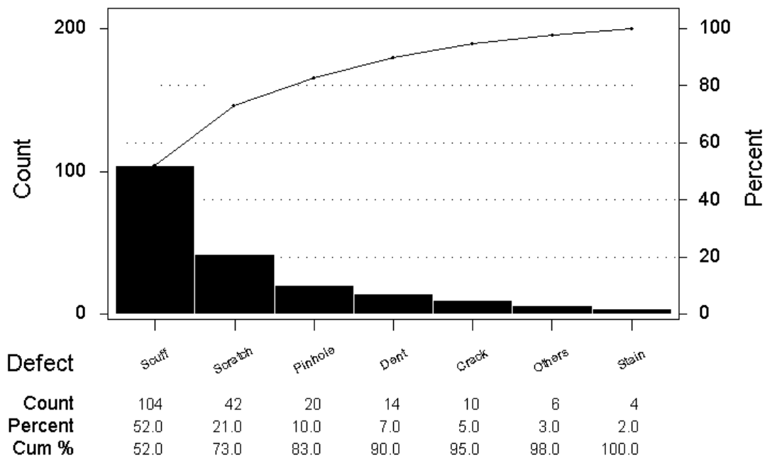
Pareto chart of Auto Grill Defects
